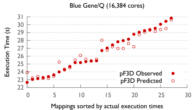
Figure 14: Comparing predicted values with observed values for pF3D on 16,384 cores. Highly accurate ordering of mappings is obtained.
