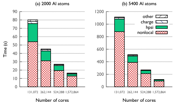
Figure 6. Timing breakdown of dominant terms in iteration loop time for (a) 2000 Al atoms and (b) 5400 Al atoms, using the ETRS propagator and distributed A_{nl} . The “nonlocal” label refers to the time evaluating all terms related to the non-local pseudopotential (energy, Hamiltonian and forces), ‘other’ refers to the contribution of all other terms in the potential to the Hamiltonian, and ‘charge’ refers to the calculation of the electronic charge density from the orbitals.
